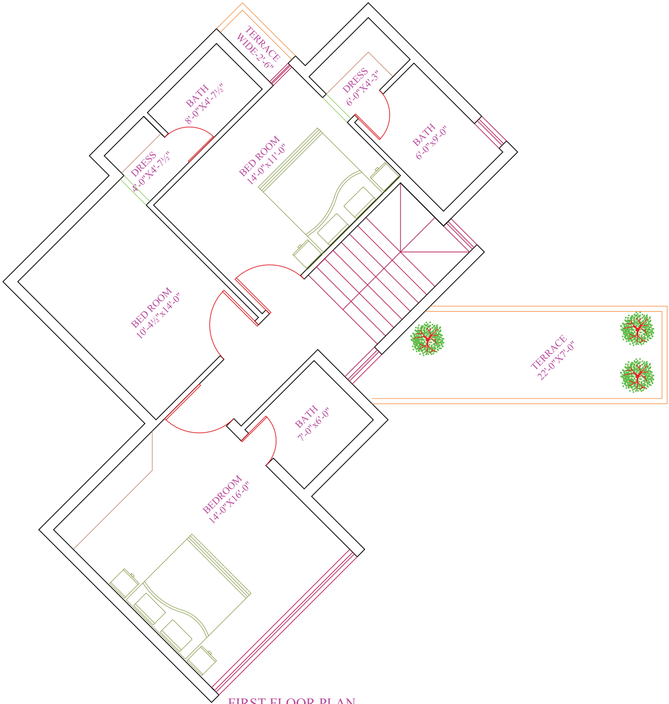
FIRST FLOOR PLAN (972.317 square ft.)
