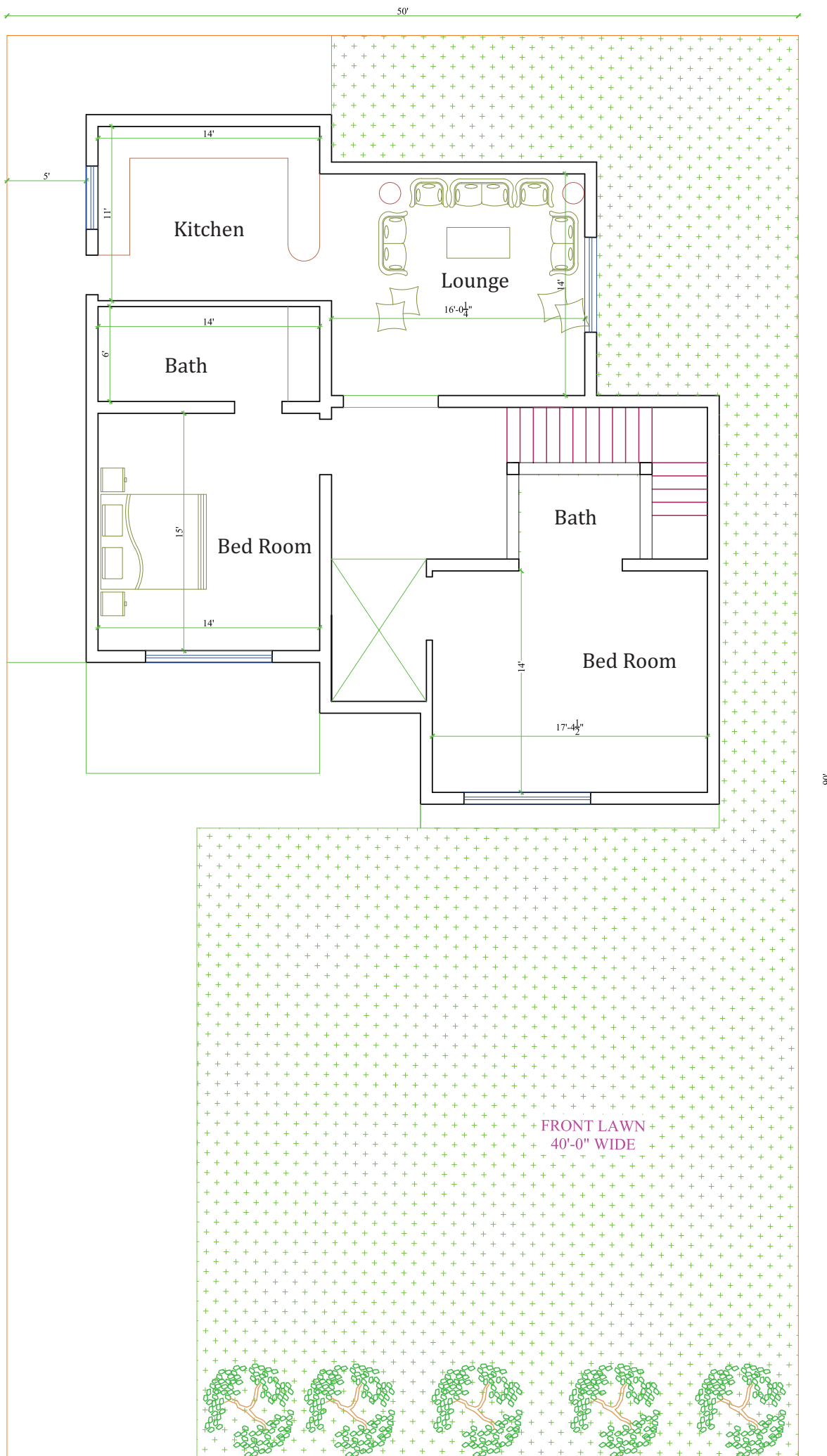
GROUND FLOOR PLAN (1450.00 square ft.)
